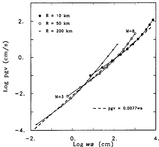
Fig. 11. Peak Wood-Anderson response and peak velocity calculated at distances of 10, 50 and 200 km, using the stochastic model described in the caption to Fig. 10. At each distance, the calculations were made for moment magnitudes ranging in 0.5 unit steps from magnitude 3 to magnitude 8. The heavy dashed line is the relation found from data (Boore, 1983, figs. 8 and 9). A similar plot for the response of a seismoscope is given in Boore (1984, fig. 5).
