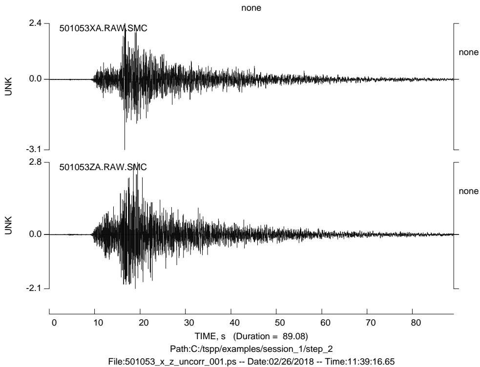
Figure 1. Plot of unprocessed acceleration time series. Note that the grainy appearance is a result of the time series values being replaced by an average value per pixel, thus greatly speeding up the plotting and reducing the file size.
