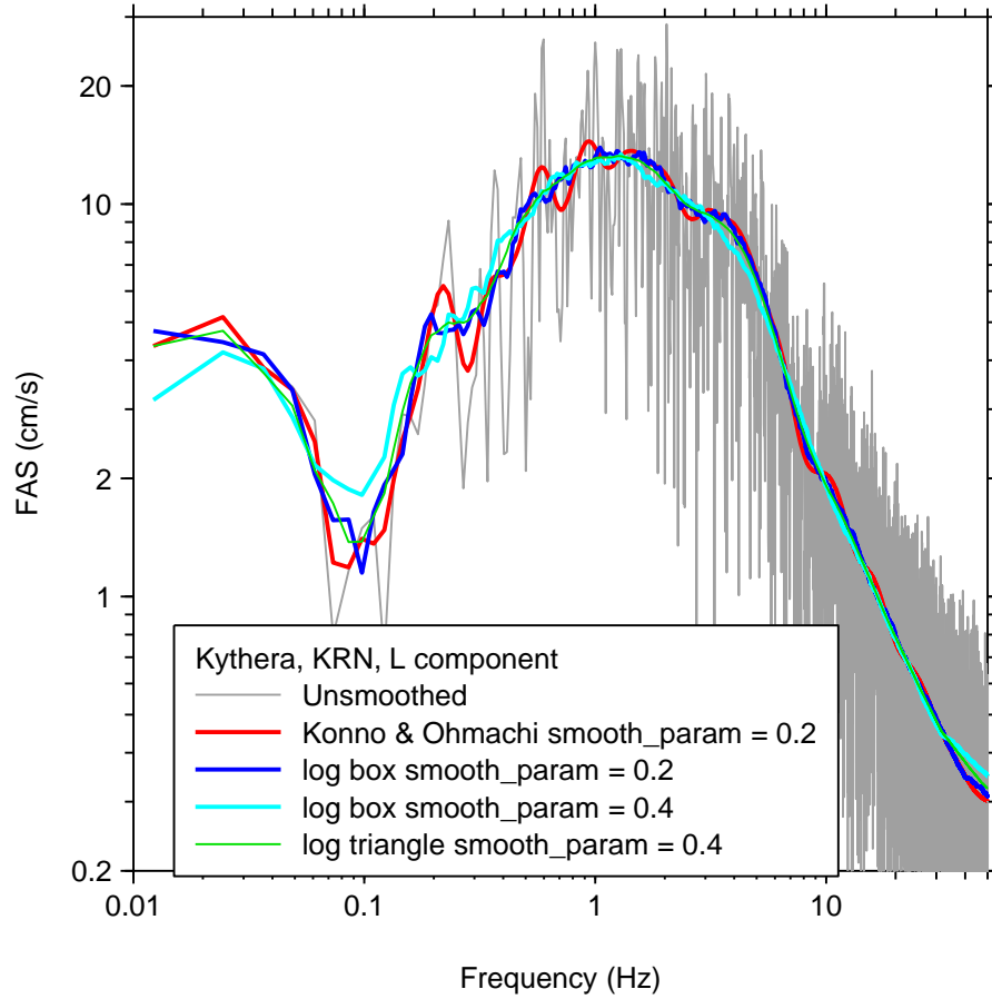
Figure 9. FAS without smoothing and with frequency-dependent smoothing.
