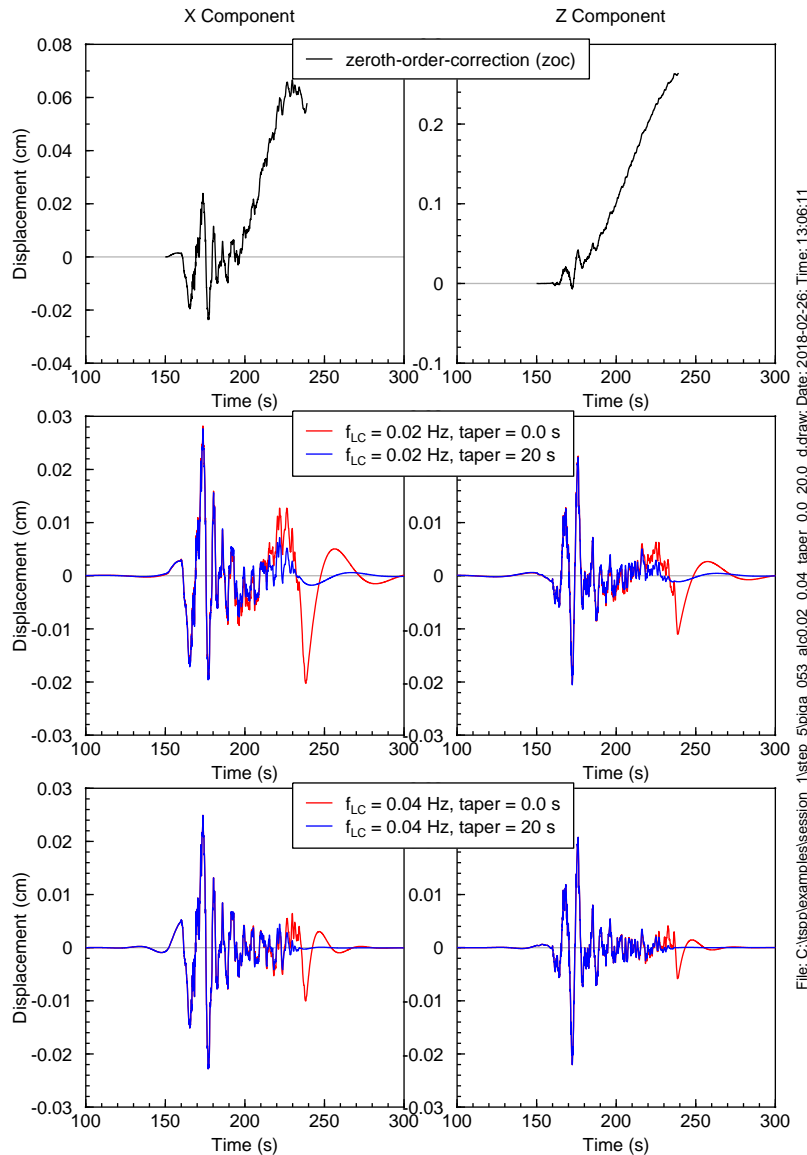
Figure 4. Plot of displacement time series from zoc (top) and filtered processing, with and without tapers where the training zeros are added to the data.
